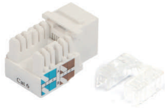
TOM-KJ-39-C5E/C6 CAT5E/CAT6 UTP Keystone Jack Punch Down Type, 90 Degree
